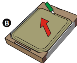
FIGURE 1. UGR-E BIB Operating Instructions, for Heater with Hydrogen Generating Warning
